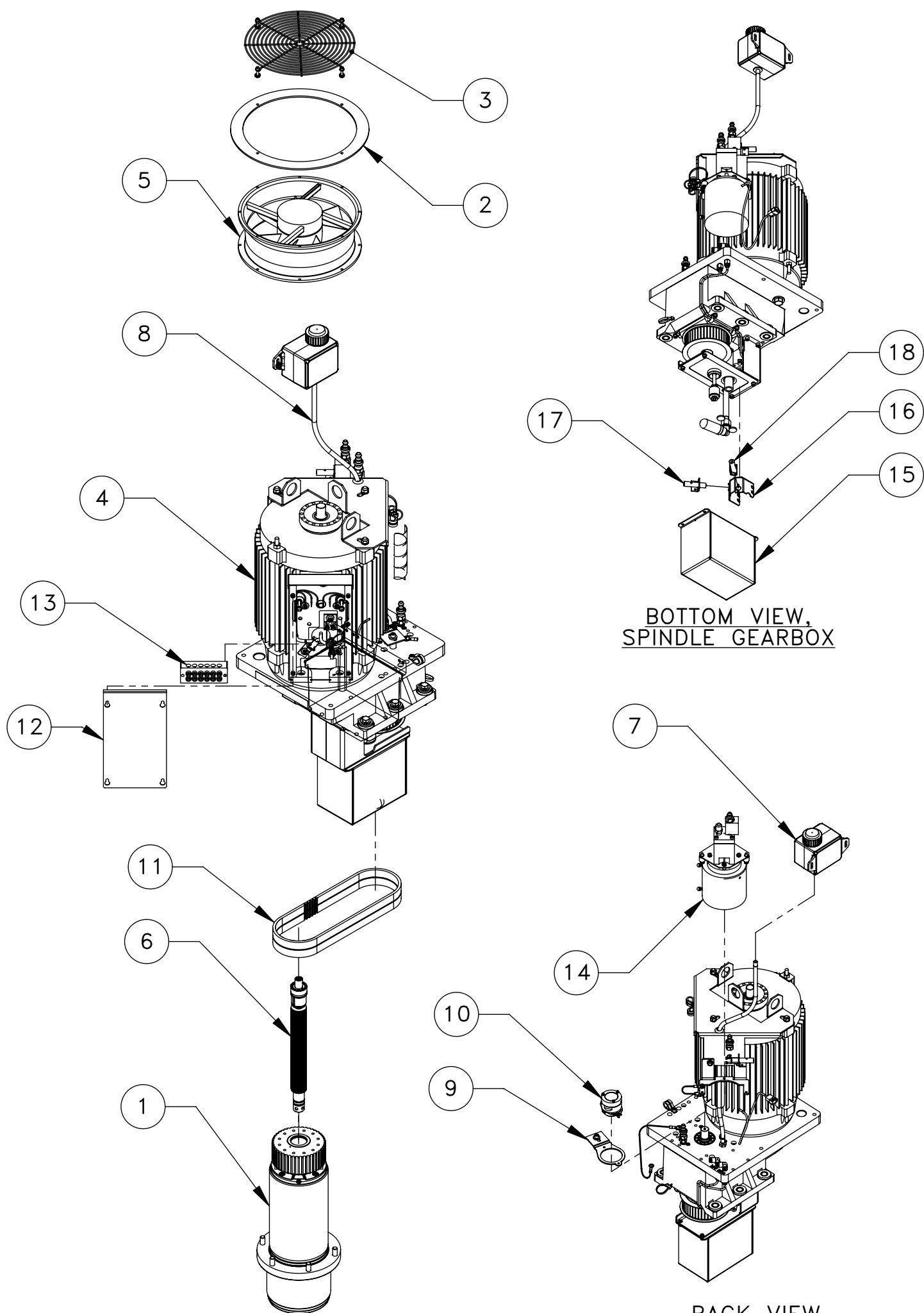
BACK VIEW, SPINDLE GEARBOX
